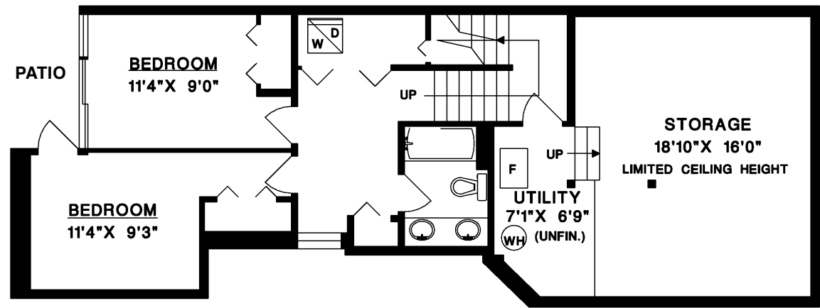
LOWER FLOOR
